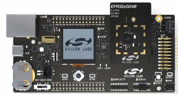
xG24-PK6010A(+20 dBm)
